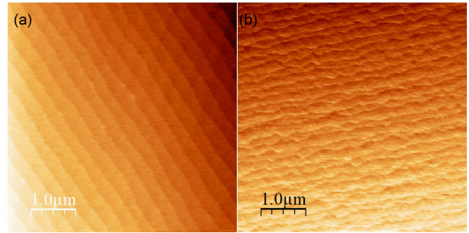
FIG. 2. AFM images of (0001) sapphire surface annealed at 1200 °C during 4 h presenting terrace-step structures. (a) Substrate 1 annealed with nitrogen presents well-defined step of 2-Å height, corresponding to the minimum distance between the oxygen layers in the sapphire lattice (1/6 lattice parameter). (b) Substrate 2 annealed with oxygen leads to step bunching of 2-6 Å and faceted step edges.
