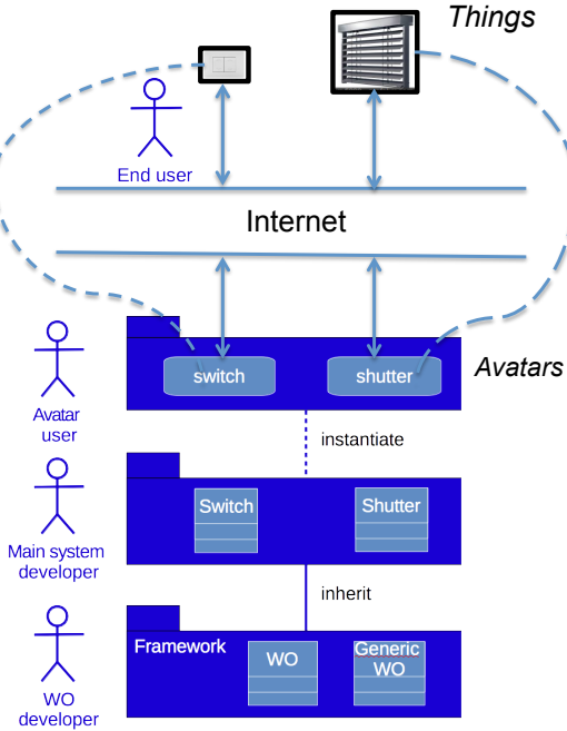
Figure 5: WIoT architecture
