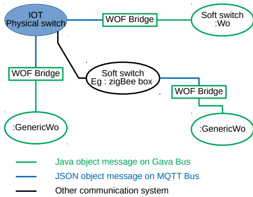
Figure 13: An IoT object, like a switch can be connected to WOF according to 3 ways: a) the thing can communicate using our MQTT protocol and its avatar exists in the WOF, b) the thing can communicate using our MQTT protocol but its avatar does not exist in the WOF, c) the thing cannot communicate using our MQTT protocol
