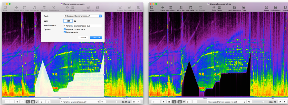
Figure 13. EAnalysis: SuperVP filter from a graphic shape.
