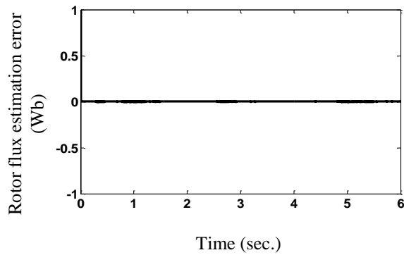
Figure 3. Performance in Benchmark 1 of the proposed observer during starting operation with load change
