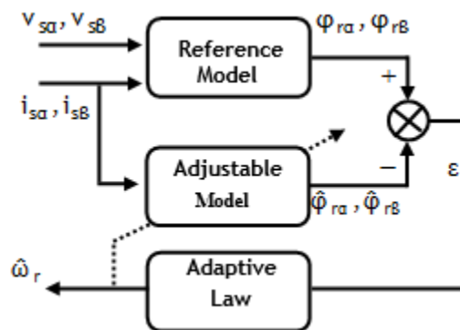
Figure 1. Block diagram of MRAS observer
