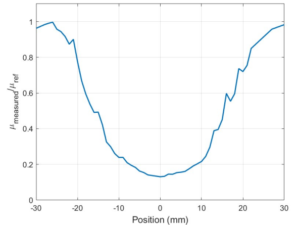
Fig. 8. Relative coercivity and the maximal permeability of the mumetal along the reference line.
