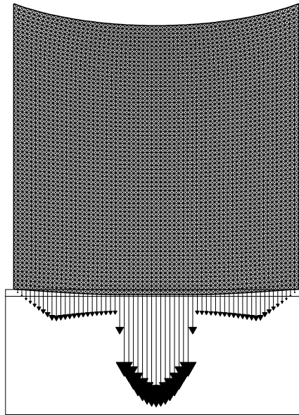
FIG. 5.5. Problem (P 4 ): Deformed mesh and interface forces for a normal compliance and unilateral constraint case for \alpha = 40 and \beta = 0.5
