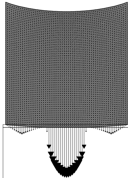
FIG. 5.6. Problem (P 4 ): Deformed mesh and interface forces for a normal compliance and unilateral constraint case for \alpha = 40 and \beta = 0
