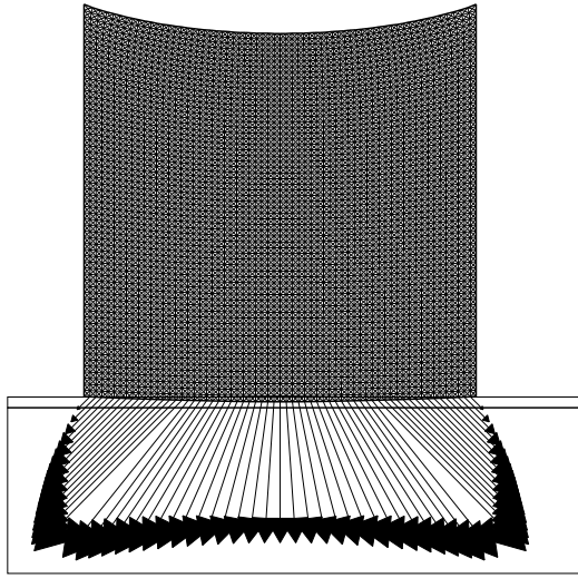
FIG. 5.8. Problem (P 2 ): Deformed mesh and interface forces for a normal compliance case with friction for \alpha = 150 and \beta = 0.5
