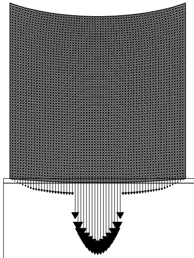
FIG. 5.3. Problem (P 4 ): Deformed mesh and interface forces for a normal compliance and unilateral constraint case for \alpha = 10 and \beta = 2
