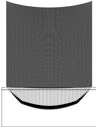
FIG. 5.2. Problem (P 4 ): Deformed mesh and interface forces for a normal compliance case for \alpha = 40 and \beta = 2
