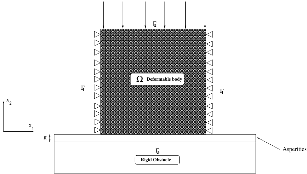
FIG. 5.1. Reference configuration of the two-dimensional body
