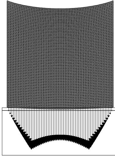
FIG. 5.4. Problem (P 4 ): Deformed mesh and interface forces for a normal compliance case for \alpha = 150 and \beta = 0.5
