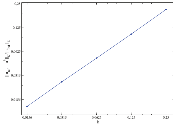
FIG. 5.9. Problem (P 2 ): Energy norm errors for frictional contact with normal compliance
