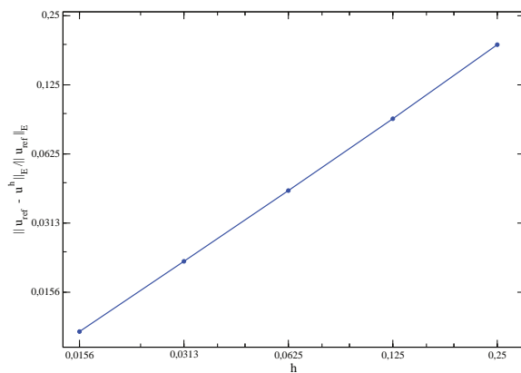
FIG. 5.7. Problem (P 4 ): Energy norm errors for frictional contact with normal compliance and unilateral constraint
