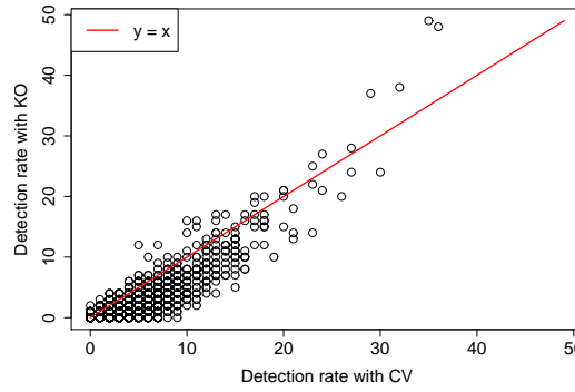
(d) Comparison of detection rates of noisy covariates for the revised knockoffs method with gaps-threshold and for cross validation.
