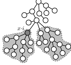
Figure 9: The disjoint values property states that for every position x \cdot i , the intersection of the grey zones is present in the last configuration for x \cdot i appearing in the run.
