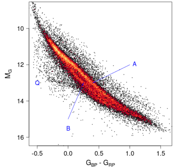
Fig. 13. Gaia HRD of white dwarfs with \sigma_\varpi/\varpi < 5\% (26 264 stars), with letter labels to the features discussed in the text.
