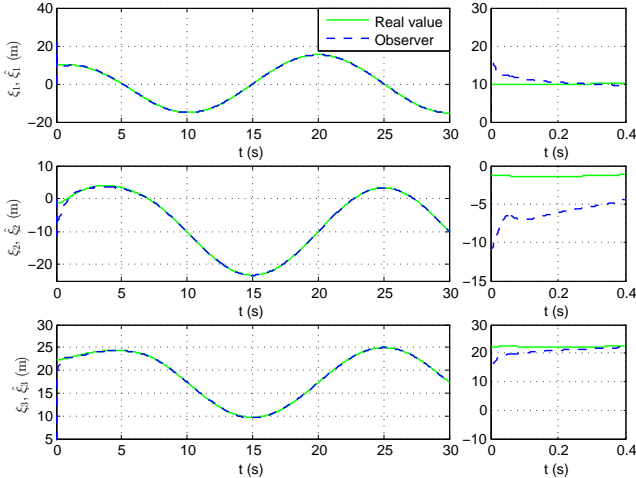
Fig. 2. Estimated and real position expressed in \{T\} versus time (s) (LEFT) and zooms (RIGHT)
