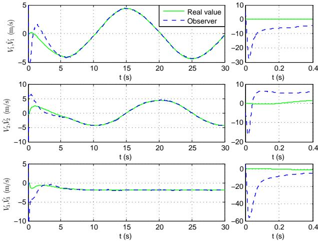
Fig. 3. Estimated and real linear velocity ( m/s ) expressed in \{B\} versus time (s) (LEFT) and zooms (RIGHT)
