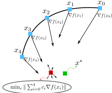
Figure 5: Regularized nonlinear acceleration can be viewed as finding the center of mass (in red). The gradients represent the forces and the green point is the real critical point x^* , whose gradient is equal to zero.
