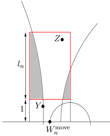
Figure 5: The red rectangle represents \text{Rec}(g_n^{\uparrow, 1}; 1, l_n) , where g_n^{\uparrow, 1} = W_n^{\text{move}} + (0, 1) , which is partially covered by the history set H_n (the gray regions). By definition of l_n the area of \text{Rec}(g_n^{\uparrow, 1}; 1, l_n) \setminus H_n is equal to 1/2 . The vertex Y is an element of W_n^{\text{stay}} while Z is a Poisson point of \mathcal{N}_{n+1} . This picture illustrates the tricky situation occurring in the proof of Lemma 3.5: although I_{n+1} = 1 , W_{n+1}^{\text{move}}(2) is not larger than W_n^{\text{move}}(2) + 1 since h(W_n^{\text{move}}) = Y .
