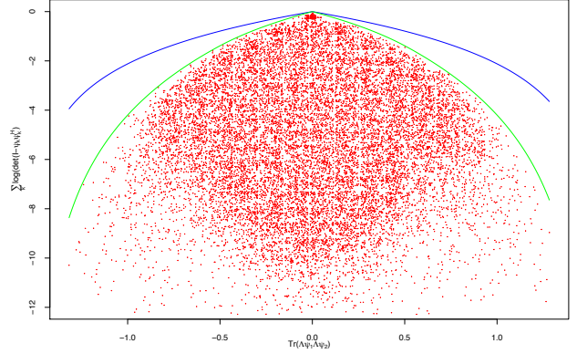
Fig. 1. graph of -I_\eta(x) seen as an upper envelope. Upper curve: the upper bound computed in [5]
