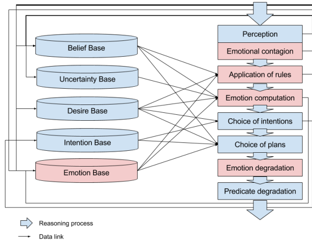
Fig. 2. Schema of the developed architecture with the addition of emotions
