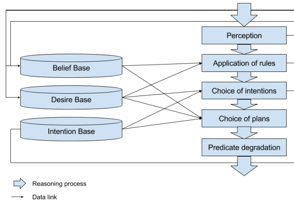
Fig. 1. Schema of our cognitive architecture
