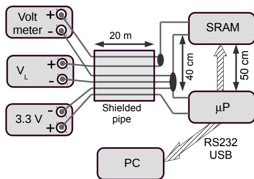
Figure 1. Schematic of connections and length of the cables. A 100- \mu\text{F} capacitor was placed between the power supply and ground in the microcontroller board, and a smaller one (100 nF) in the SRAM board. The cable shield was connected to the ground output of the 3.3 V power supply.
