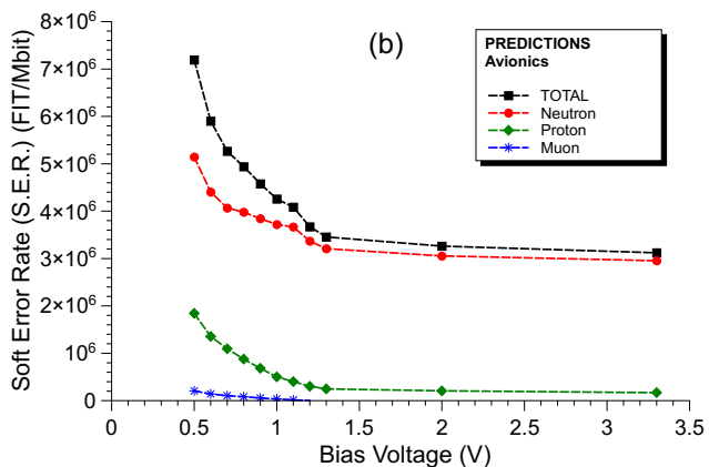
Figure 7. Calculated SER vs. bias voltage at the avionic level. (a) SBU to 6-bit MCU SER. (b) SER distinguishing the contributions of protons, neutrons and muons
