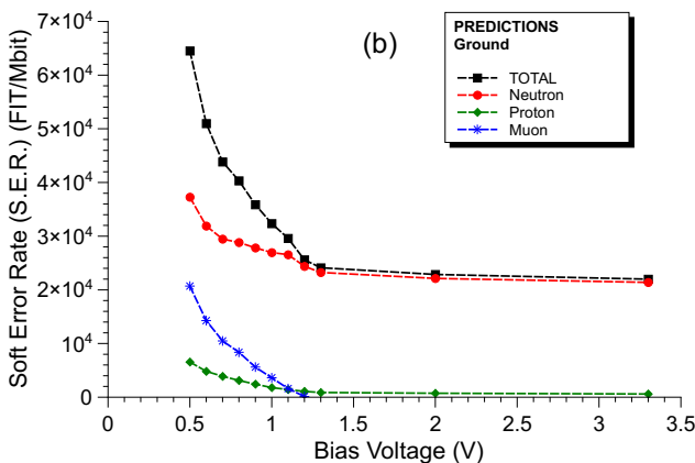
Figure 6. Calculated SER vs. bias voltage at ground level. (a) SBU to 6-bit MCU SER. (b) SER distinguishing the contributions of protons, neutrons and muons
