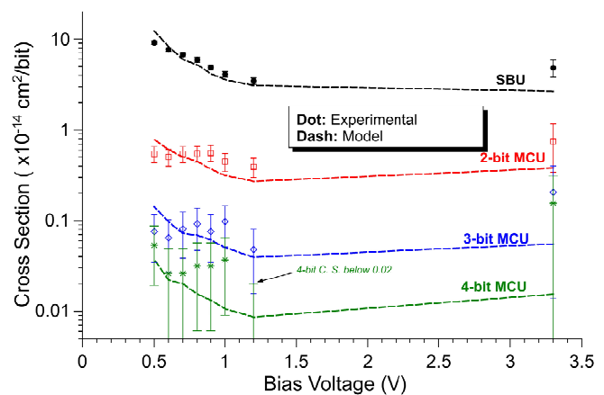
Figure 2. Cross sections of the 90-nm memory studied, for different voltage levels. Dots indicate experimental measurements, whereas the dashed line indicates the predictions issued from MUSCA-SEP3.
