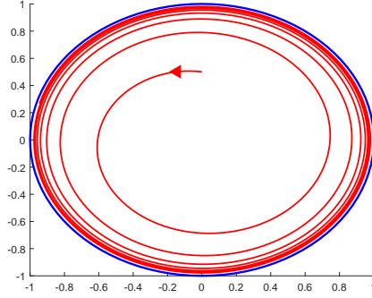
FIGURE 3. B(r) = e^{-r} - \frac{2}{r} .
