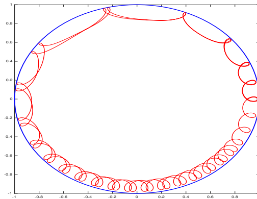
FIGURE 1. A trajectory obtained with a magnetic field on the unit disc that is strong near the boundary with a non-integrable tangential derivative:
