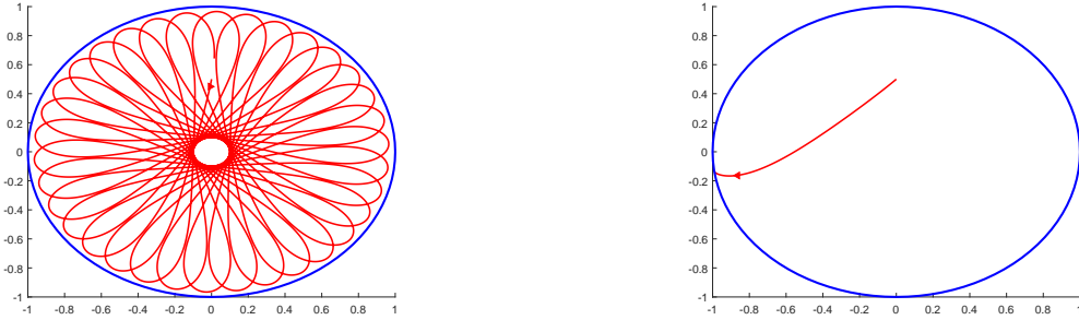
FIGURE 4. B(r) = \ln^2(1-r) : the particle is confined or not.
