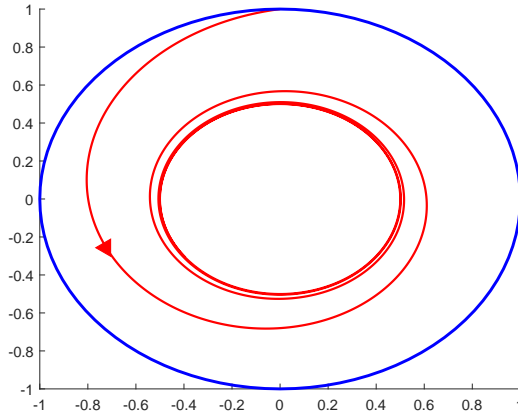
FIGURE 6. B(r) = e^{-r} - \frac{2}{r} .
