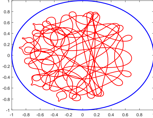
FIGURE 2. A trajectory obtained with a magnetic field on the unit disc that strongly oscillates near the boundary:
