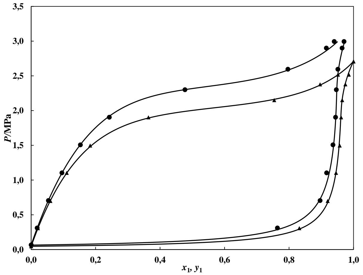
Figure 2. P - x - y data for the R116 (1) + n-pentane (2) system. ▲, T = 288.25 K; ●, T = 296.24 K; —, PR-EOS based model.
