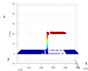
Fig. 13. Best representation on the Reg scene using classical beamforming (a), Capon beamforming (b), MUSIC (c), CS (d) and our tomographic 3D inversion (e).
