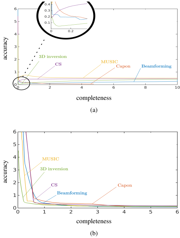
Fig. 15. Accuracy vs. completeness for classical beamforming, Capon beamforming, MUSIC, Compress Sensing and our 3D Inversion algorithm. In (a) the evaluation is done on the Reg scene 6 and in (b) on the TSX scene 6.
