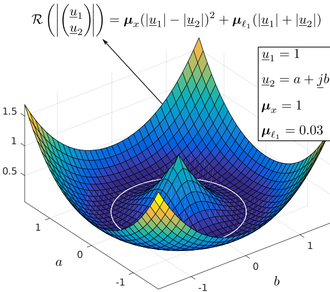
Fig. 4. Illustration of the non-convexity of spatial regularizations expressed on the modulus of the complex reflectivities.
