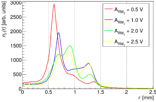
Fig. 8. Antiproton radial profiles after the single step \bar{p} RW compression at f_{RW_2} = 3 MHz for different drive amplitudes A_{RW_2} . The ring structures are due to the centrifugal separation caused by a delay between turning off the RW drive (heating) and particle extraction. Lower amplitudes favor smaller \bar{p} tails.
