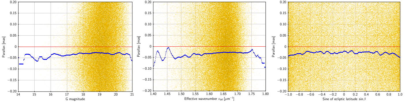
Fig. 7. Parallaxes for the full quasar sample plotted against magnitude ( left ), colour ( middle ), and ecliptic latitude ( right ). Because of the chosen scale, only about one-third of the data points are shown as yellow dots; the blue curves are the running medians.
