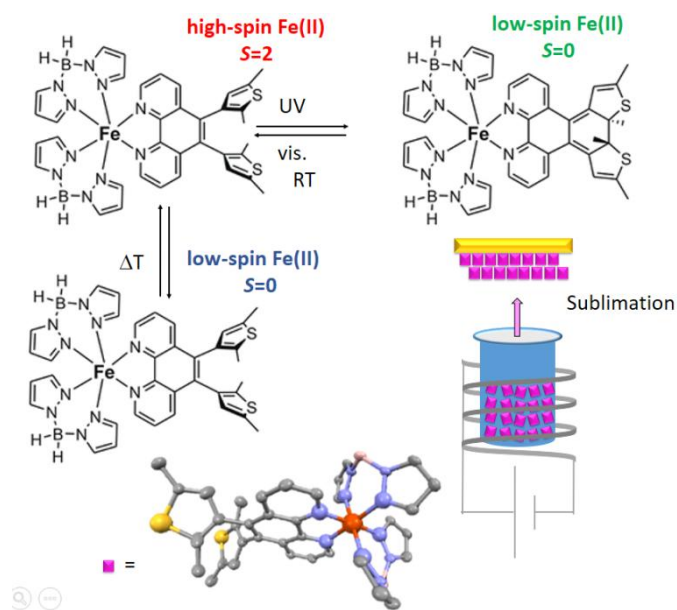
Figure 1. Molecular structure of the [\text{Fe}^{\text{II}}(\text{H}_2\text{B}(\text{pz})_2)\text{phen}^*] complex and schematic representation of the UHV sublimation process (bottom). Control of the spin state by room-temperature photocyclization of phen * ligand and by temperature (top).
