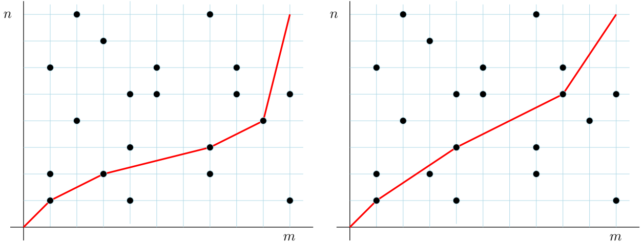
Figure 2: Realizations of \mathcal{L}_{(m,n)}^{(2,1)} (left) and \mathcal{L}_{(m,n)}^{(3,2)} (right) for (m,n) = (10,8) and the same sampling of \Xi (points of \Xi are represented with \bullet ). Here we have \mathcal{L}_{(m,n)}^{(2,1)} = 4 , \mathcal{L}_{(m,n)}^{(3,2)} = 3 . In both pictures one of the maximizing paths is drawn in red.
