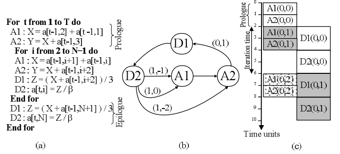
Fig. 2. The Jacobi algorithm after r(A1 \rightarrow A2) = (0, 1) : (a) code, (b) MDFG, (c) static schedule
