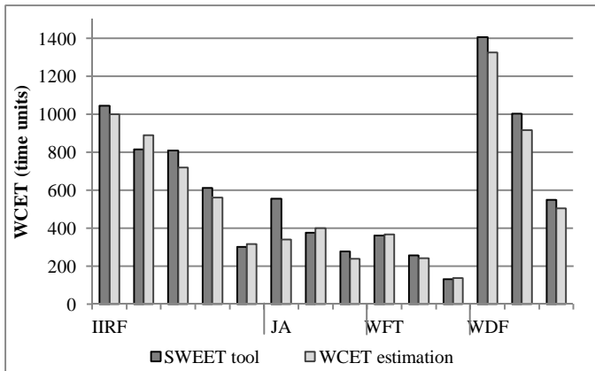
Fig. 5. Benchmark WCETs in terms of SWEET tool and WCET equation
