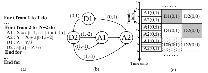
Fig. 3. The Jacobi algorithm provided by the delayed MR: (a) code, (b) MDFG, (c) static schedule
