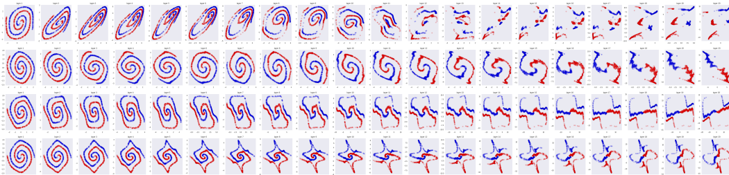
Figure 3: Evolution of the spatial configuration of data points through the 20 residual units. From top to bottom: ResNet without shared weights, ResNet with shared weights, Data-driven Symmetric ResNet with shared weights, Domain-driven Symmetric ResNet with shared weights.
