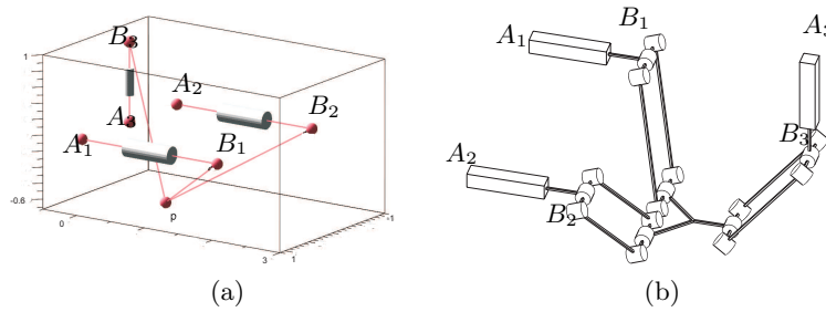
FIGURE 5: Configuration of Hybridglide : (a) simplified; (b) real.
