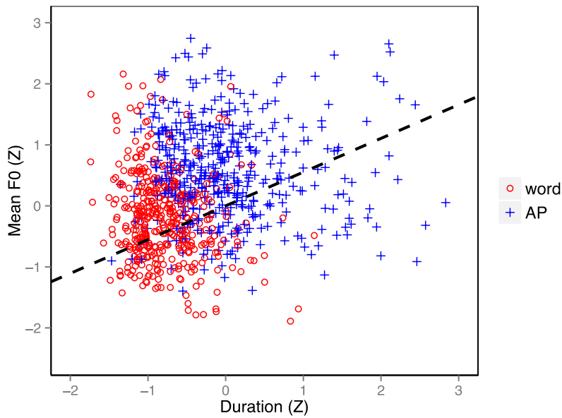
Figure 4. Scatterplot of nucleus duration and nucleus mean f_0 by boundary type. All values are standardized by speaker (z-score). The dashed line represents the eigenvector of the linear discriminant.
