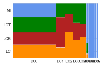
(b) Final clusters
