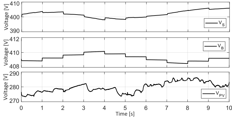
Figure 3. Voltage on supercapacitor V_S , battery V_B and PV array V_{PV} respectively. Voltage V_{C_7} is related to the power generated in the PV, which highlights the intermittent feature of this renewable energy source.
