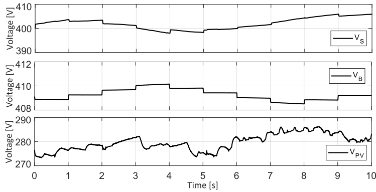
Figure 3. Voltage on supercapacitor V_S , battery V_B and PV array V_{PV} respectively. Voltage V_{C7} is related to the power generated in the PV, which highlights the intermittent feature of this renewable energy source.
