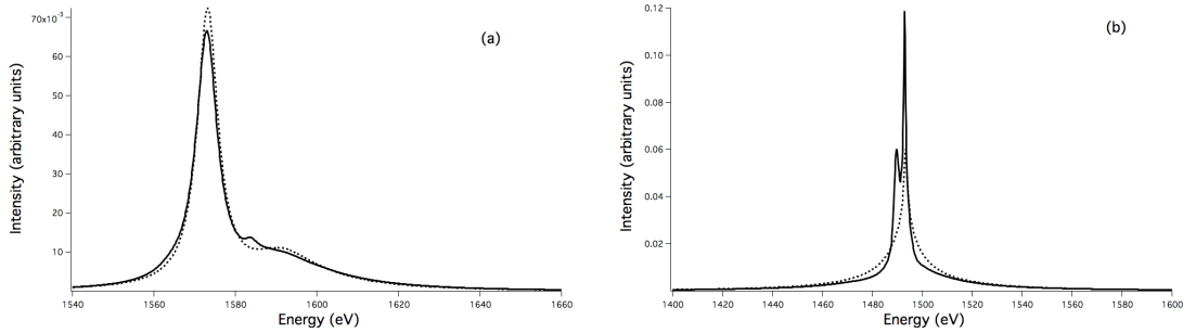
FIGURE 6. Spectral line shape of Ne-like aluminum with N_e = 3.625 \times 10^{22} \text{ cm}^{-3} and T_e = 20 \text{ eV} of a) transitions nl-1s with ionic Stark effect (full line) and without ionic Stark effect (dotted line); b) transitions 2p-1s with interference effects (full line) and without interference effects (dotted line)
