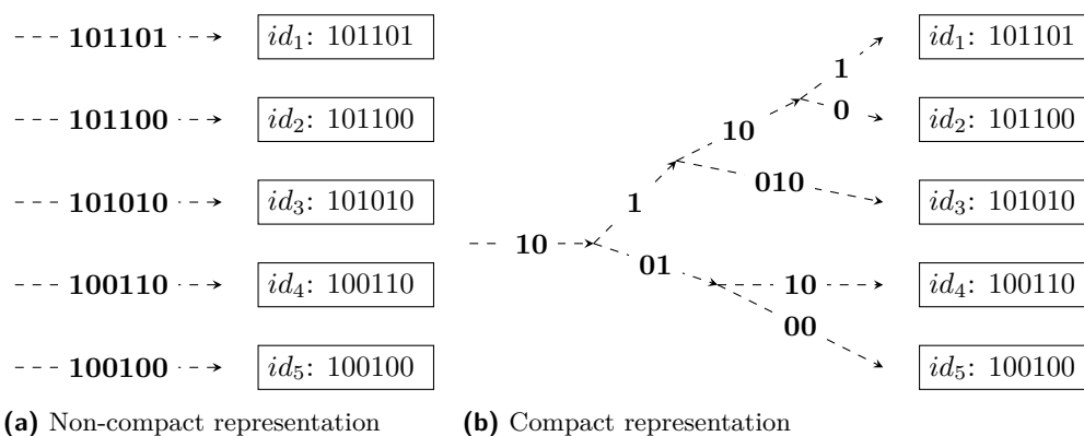
■ Figure 2 Difference between non-compact and compact representations of k different values (ids), indicated by the number of bits used as labels
