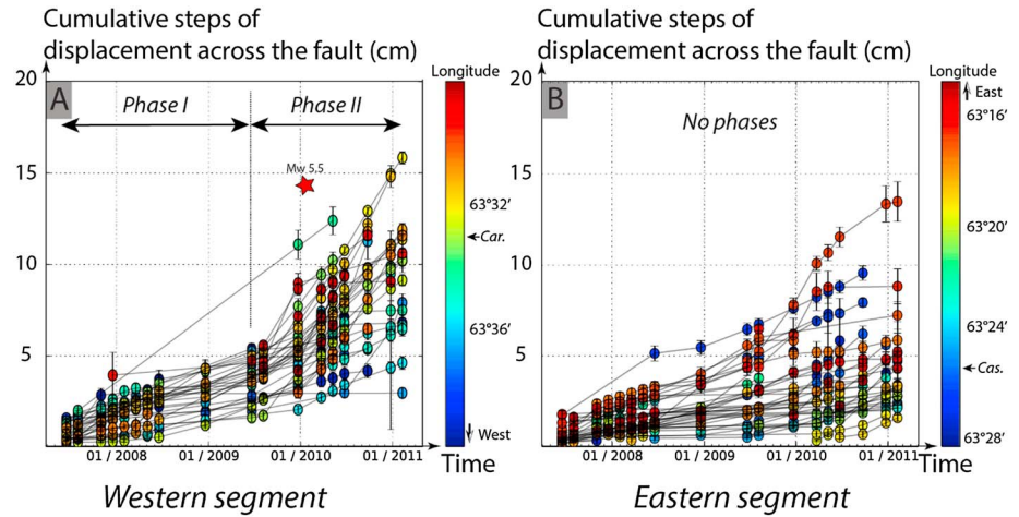
Figure 9. Cumulative displacement steps (in centimeters) across the El Pilar fault for each time step of the time series. Cumulative step estimation involves fitting the times series values weighted with RMS for each 480 m (or 16 pixels). For each estimation using 1, the standard deviation (error bars) is plotted. The dot color corresponds to the longitude along the fault. (a) Cumulative displacement steps (in centimeters) across the western segment. The average velocity of the two phases was defined using linear regression between cumulative displacement and the date at each longitude along the fault. Red star marks the M_w 5.5 earthquake in January 2010. (b) Cumulative displacement steps (in centimeters) across the eastern segment. \chi^2 value for each dot is plotted in Figure S9. Car., Cariaco and Cas., Casanay.
