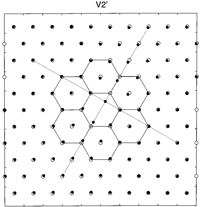
FIG. 3. The new vacancy configuration V2' obtained for the box size (L_x, L_y) = (5, 6\sqrt{3}/2)ta with t=5 , presented as in Fig. 1. In the case \lambda/a = 0.25 this new vacancy type has a lower energy than the vacancy V2 shown in Fig. 1(c). One can see that the two mirror planes (dotted lines) cross at a flux line and not at the initial vacancy position. Thus, the initial vacancy position is no longer the center of symmetry.
