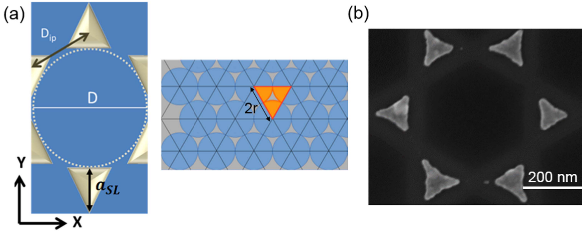
Figure 3. (a) Scheme for the FDTD simulation of the unit cell with the geometrical parameters of a metallic NP and an overview of the NP array. (b) SEM image of a part of Ag-NP array obtained from SiO 2 nanospheres with diameter D of 400 nm.
