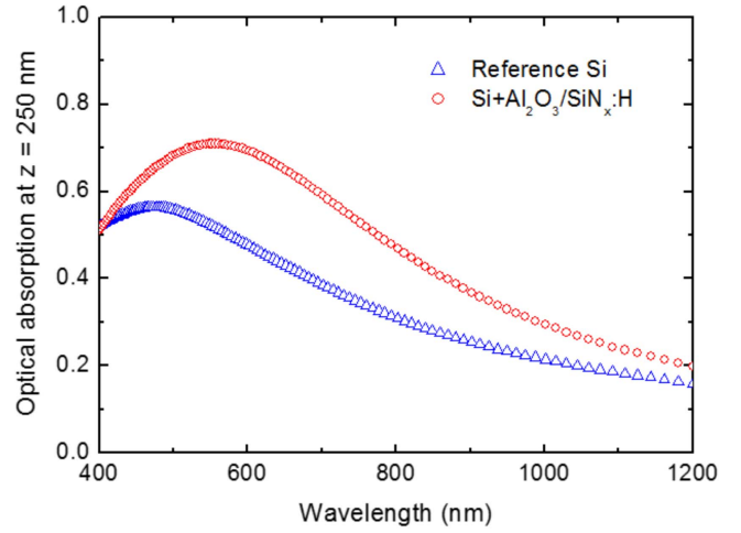
Figure 6. FDTD simulations of optical absorption at z = 250 nm for (a) Si substrate and (b) \text{Si}+\text{Al}_2\text{O}_3/\text{SiN}_x\text{:H} stacks.
