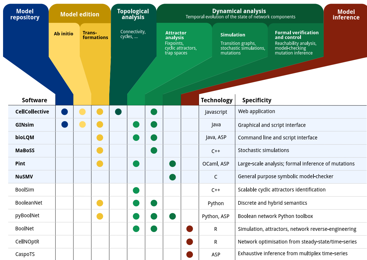
Figure 1: Feature matrix and characteristics of a range of software tools devoted to the qualitative modelling and analysis of biological networks: CELLCOLLECTIVE [23]; GINSIM [33]; BIOLQM [32]; MABOSS [48]; PINT [37]; NUSMV [11]; BOOLSIM [20]; BOOLEANNET [3]; PYBOOLNET [26]; BOOLNET [31]; CELLNOPT [51]; CASPOTS [36]. The current CoLoMoTo Docker (2018-03-31) ships the software indicated with a bold font and a light blue background. “Model repository” refers to searchable databases of models; “Model edition” refers to the features related to creating and modifying a qualitative model, where “ ab initio ” refers to the interactive model building from scratch, and “transformations” refers to operations such as mutations, Booleanization, model reduction, etc. “Topological analysis” refers to the extraction of features from the regulatory graph, such as the different feedback cycles, graph theory measures, etc. “Dynamical analysis” refers to properties related to the state transition graph of Boolean/multi-valued networks, where “Attractor analysis” refers to the identification of stable states, cyclic attractors, and related features; “Simulation” refers to the sampling of trajectories within the state transition graph, possibly parameterized with stochastic rates and mutations; “Formal verification and control” refers to exhaustive analyses for assessing strictly temporal properties, such as reachability, and deducing mutations for controlling the system. Finally, “Model inference” refers to the derivation of Boolean/multi-valued network which are compatible with given properties and observation data.
