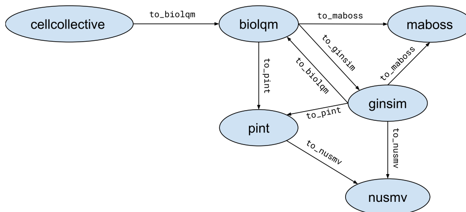
Figure 2: Supported model conversions between Python modules.
