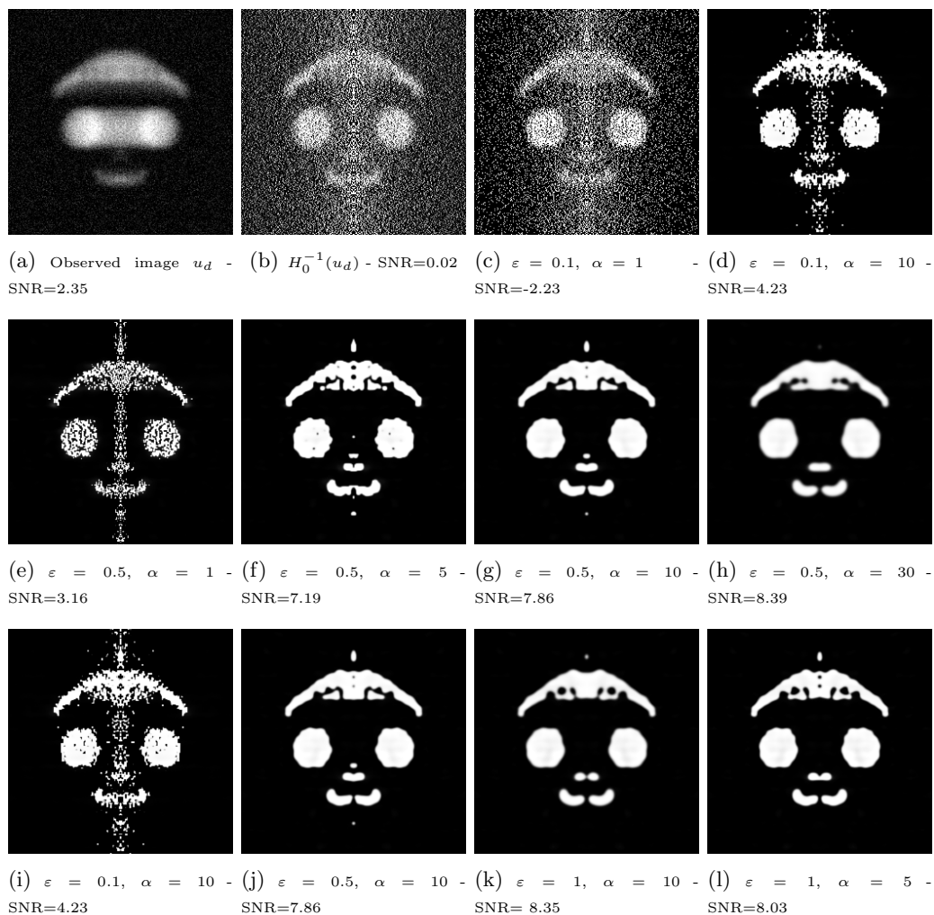
Figure 3.5: Blur and noise (SNR = 2.35) - s = 0 ( L^2 norm), simulations with different values of \varepsilon and \alpha
