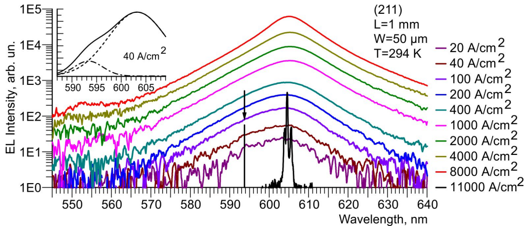
Fig. 6. EL spectrum of (211) laser at different current densities. A strong superlinear growth of the intensity is observed at current densities above 400 \text{ A/cm}^2 . The band of stimulated emission and lasing is Stokes-shifted from the bandgap feature resolved at low excitation densities. The insert shows the deconvoluted EL spectrum at 40 \text{ A/cm}^2 in linear scale revealing a bandgap emission with the maximum at 603.5 \text{ nm} (dashed line) and emission at a shorter wavelength with the maximum at 594 \text{ nm} (dash-dotted line). Lasing spectrum is not to scale.
