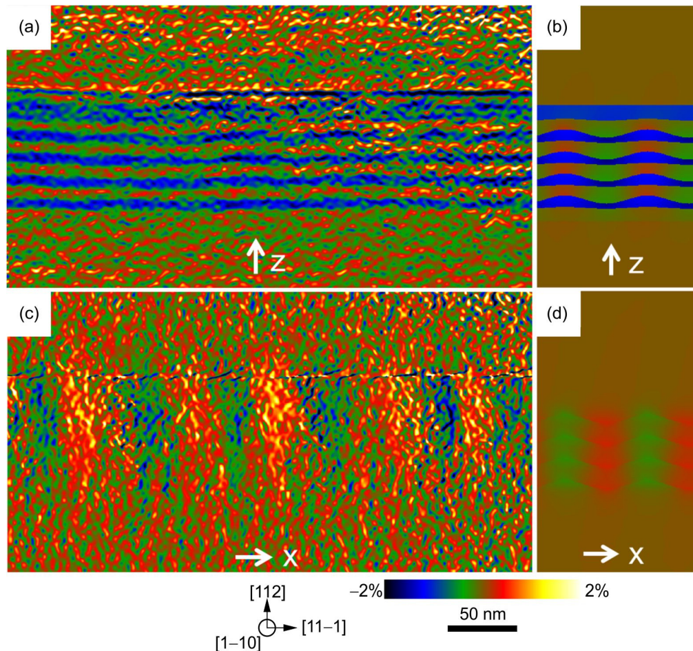
Fig. 2. (a) Out-of-plane \epsilon_{zz} and (c) in-plane \epsilon_{xx} strain distributions in the gain medium of the (112) structure which contains four tensile strained nominally 4-nm thick \text{In}_{0.4}\text{Ga}_{0.6}\text{P} layers. Strain was extracted with respect to \text{Ga}_{0.21}\text{Al}_{0.30}\text{In}_{0.49}\text{P} lattice with a 4-nm spatial resolution by applying moiré by specimen design technique in cross-section (1-10). (b) Out-of-plane \epsilon_{zz} and (d) in-plane \epsilon_{xx} strain distributions obtained by finite element method modelling. Note column-like \epsilon_{xx} strain variation both in (c) and (d).
