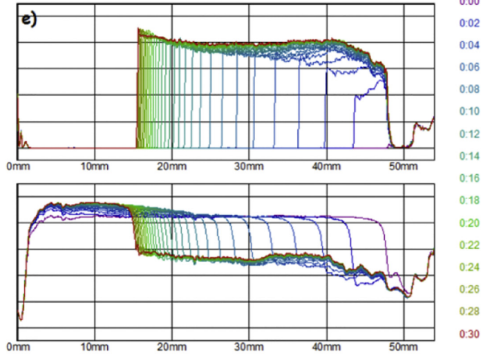
Fig. 3. Turbiscan profiles in limewater of calcite suspension unadmixed (a), admixed with different superplasticizer concentrations (0,1% for b) and 1% for c). (d) and (e) correspond to Turbiscan profiles of unadmixed suspensions in \text{NaNO}_3 and \text{Na}_2\text{SO}_4 solutions at I = 171 mmol/L, respectively. Each curve corresponds to a different analysis time, from 0 to 30 min.
