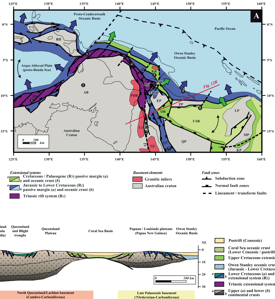
Figure 12. Rifting evolution of the Coral Sea region since the Permian to the early Tertiary. (a) Nonpalinspastic tectonic evolution showing the overprint of the three extensional megacycles along the northern margin of Australia. Numbers refer to stratigraphic columns displayed in Figure 11. (b) Reconstruction of the Coral Sea region prior Cenozoic compression, based on deep geophysical data of Ewing et al. (1970). The line shows the relationships between the various rifted domains. Section location is indicated in Figure 12a. Abbreviations: AB: Arafura Basin, BB: Bonaparte Basin, BH: Bird's head, BL: Bosavi Lineament, BT: Bligh Trough, CI: Coen Inlier, CSB: Coral Sea Basin, EP: Eastern Plateau, EPaR: East Pandora Ridge, GI: Georgetown Inlier, KI: Kubor Inlier, LP: Louisiade Plateau, NF: Nubura fault, OB: Osprey Basin, PaR: Pandora Ridge, PDR: Peninsula-Daru Ridge, PR: Pasca Ridge, QT: Queensland Trough, QP: Queensland Plateau, and ToB: Townsville Basin.
