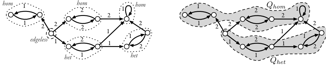
■ Figure 1 Example of G_A with the subgraphs induced by Q_{hom} and Q_{het} . For simplicity we assume that \mathbb{A} = \{a\} and we hence omit the letter a when depicting edges labeled by (i, a) .
