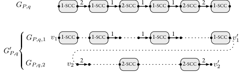
■ Figure 4 Example of construction of G'_{P,q} from G_{P,q} . The SCC are abstracted as grey boxes, labeled “1-SCC” or “2-SCC” depending on the sort of SCC they are. Edges are also labeled depending on whether they are 1-edges or 2-edges. Dotted lines are used to identify two vertices as being the same.
