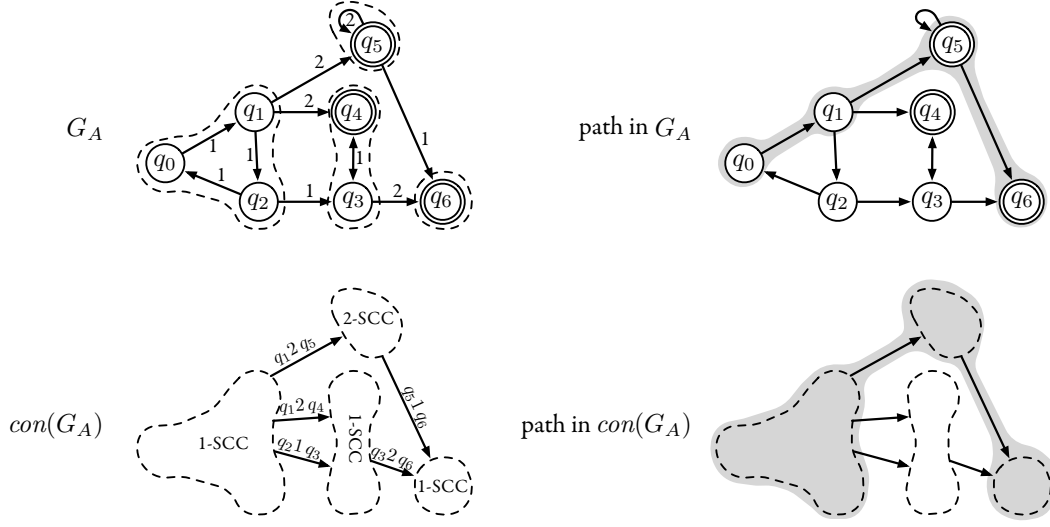
■ Figure 3 Example of path in G_A and corresponding path in con(G_A) . For simplicity, we assume that the alphabet is singleton \mathbb{A} = \{a\} , and we therefore omit ‘ a ’ in the transitions.
