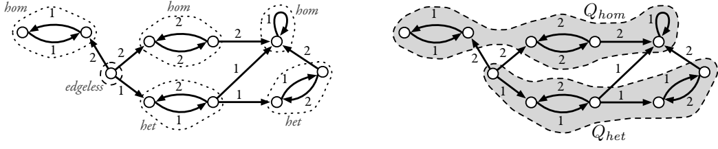
■ Figure 5 Example of G_A with the subgraphs induced by Q_{hom} and Q_{het} . For simplicity we assume that \mathbb{A} = \{a\} and we hence omit the letter a when depicting edges labeled by (i, a) .
