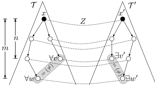
Figure 2: Zig clause of bisimulation for \text{XPath}_{\neq}^{\downarrow} .
