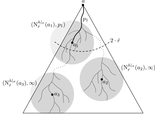
Figure 2. Idea of the abstraction of a tuple of \xi_{\mathbb{A}} , for \hat{n} = 3 . Gray balls represent non-intersecting neighborhoods of three elements a_1, a_2, a_3 . a_1 is so that \delta_{\sigma}(a, a_1) \leq 2 \cdot \hat{r} , whereas a_2 and a_3 are at distance more than 2 \cdot \hat{r} from a .
