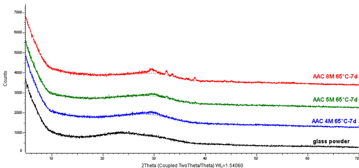
Fig. 2. XRD results of glass powder and of different alkali-activated glasses, depending on sodium hydroxide concentration (4, 5 or 8 M) and cured at 65 °C for 24 h followed by 6 days at 20 °C.
