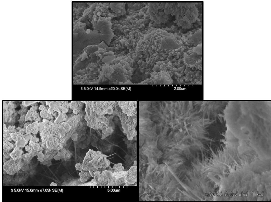
Fig. 1. (top, left and right): Cement paste of 2 M NaOH alkali-activated glass mortar cured for 24 h at 65 °C and then at 20 °C, observed at 90 days, showing the presence of needles, potentially due to C-S-H presence; (bottom): C-S-H « urchins » observed on the fracture surface of a pure Portland CEM1 standard mortar (according to EN196-1) after more than 28 days curing at 20 °C.
