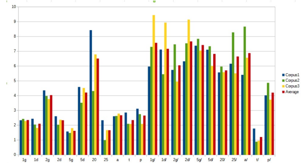
Figure 2: Relevance measures, resulting from the feature selection algorithm. The ordinate represents the average percentage of importance for each feature on the 3 corpora. The features are represented in abscissa: 1g for AU1 left, 1d for AU1 right, 2g for AU2 left, 2d for AU2 right, 5g for AU5 left, 5d for AU5 right, 20 for AU20, 25 for AU25, a, t and p represent the angles of the head rotation. 1g', 1d', ..., a', t', p' represents the times derivatives of the features.
