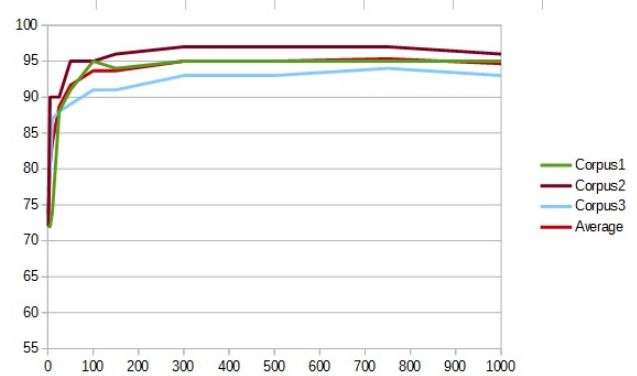
Figure 4: Classification accuracy with training and test sets of different sizes. The value on the abscissa axis represents the number of samples extracted from one video ( X ). The average curve corresponds to the average accuracy of the three corpora.
