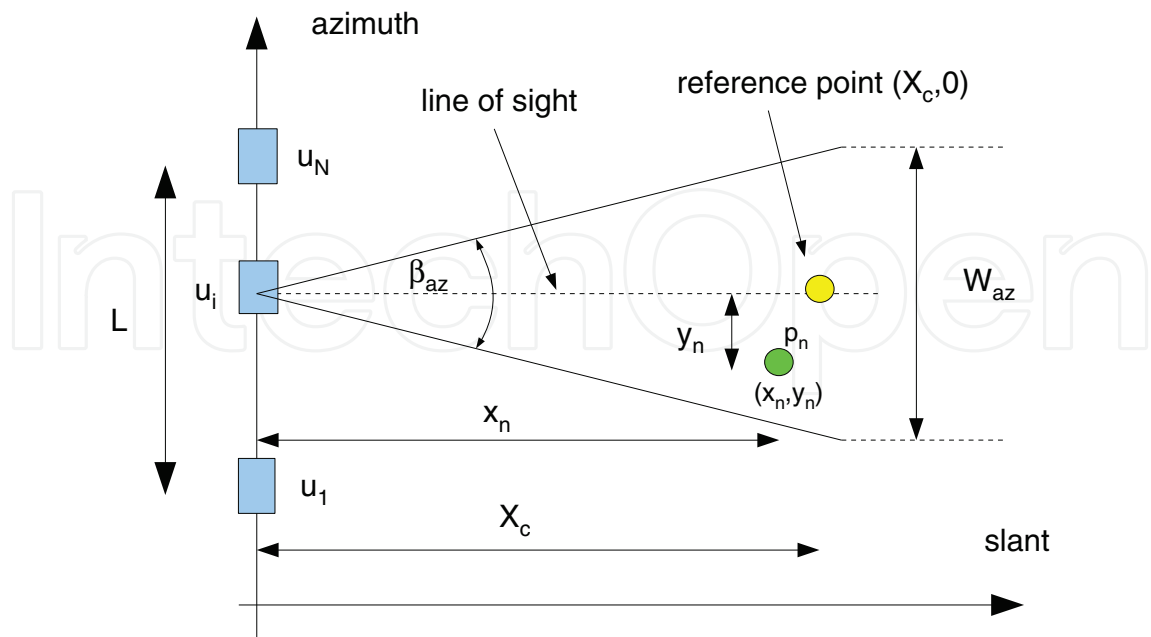
Figure 2. SAR geometric configuration in the slant-range area.
