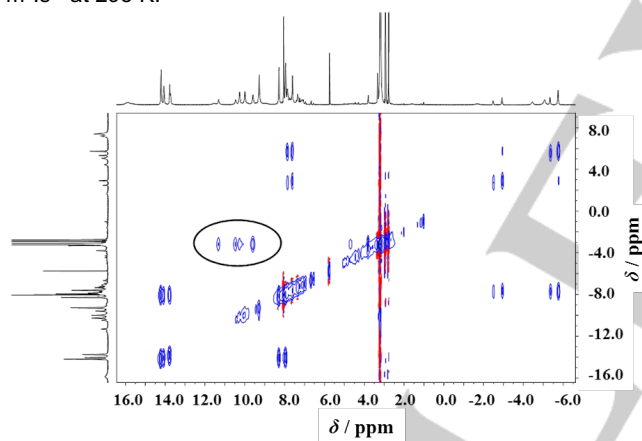
Figure 4. NOESY spectrum of 1 in N,N -Dimethylformamide- d_7 at 343 K. Cross peaks surrounded in black correspond to the correlation between protons from protonated amide arms and residual water molecules.
