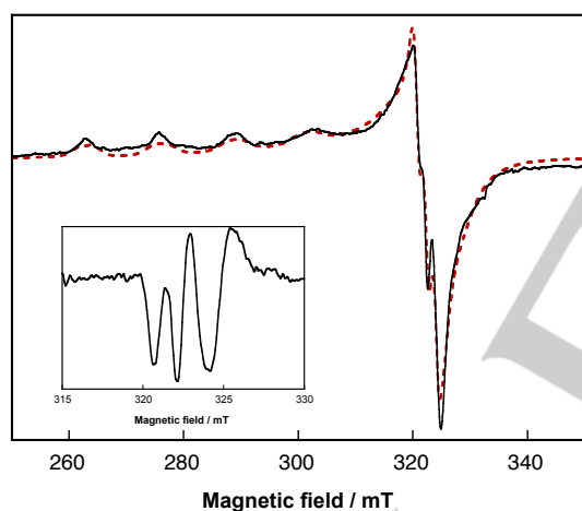
Figure 8. X-band EPR spectrum of 0.5 mM solution of chemically generated 1 + at -60°C in CH 2 Cl 2 + 10% DMF. Solid line: experimental spectrum, dotted red line: simulation. Parameters g_z = 2.356 g_y = 2.058 , g_x = 2.058 , A_{\parallel}(\text{Cu}) = 126 G, A_{\perp}({}^{14}\text{N}) = 16.8 G. Inset: Derivative spectrum. Experimental conditions: microwaves frequency 9.31 GHz, microwave power = 20 mW, modulation amplitude 0.3 mT, T = 120 K.
