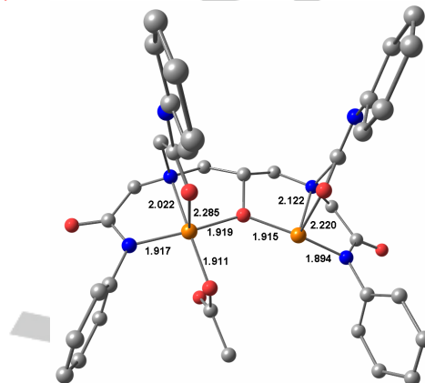
Figure 9. DFT-optimized structure and selected metrical parameters for the relevant oxidized form of 1 (form b)
