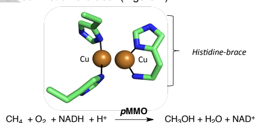
Figure 1. Structure of the dicopper active site of p MMO from Methylococcus capsulatus (Bath) and reaction catalyzed by p MMO.
