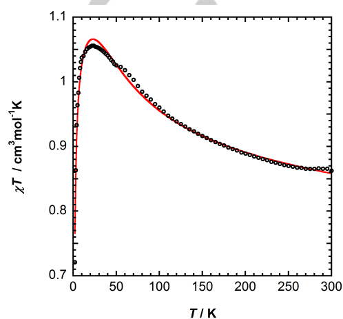
Figure 3. Temperature dependence of 1 in the solid state. Parameters from the fit: J = 53.8 \text{ cm}^{-1} , g = 2.20 , zJ' = -0.97 \text{ cm}^{-1} , C_{Cu} = -60.6 \cdot 10^{-6} \text{ cm}^3 \text{ mol}^{-1} goodness of fit R = 7.6 \cdot 10^{-5} .
