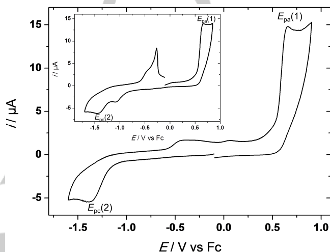
Figure 5. CV at a glassy carbon electrode of complex 1 (0.50 mM) in DMF / \text{NBu}_4\text{PF}_6 0.1 M under Argon at \nu = 0.1 \text{ V s}^{-1} , negative scanning, inset: \nu = 0.1 \text{ V s}^{-1} , positive scanning.
