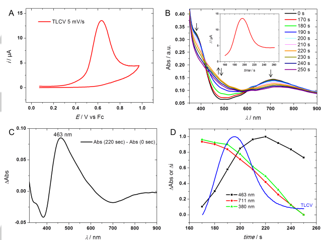
Figure 7. A) Room-temperature TLCV ( \nu = 5 mV/s) at a glassy carbon electrode of 1 (0.50 mM) in DMF / NBu 4 PF 6 0.1 M under Ar; B) 2D UV-Vis spectra of complex 1 upon TLCV experiment (5 mV/s); Inset: Variation of current with time during the CV; C) UV-Vis differential spectrum at \lambda = 463 nm between t=220 seconds t=0 seconds; D) Plots of relative absorbance vs. time during the spectroelectrochemical measurements at different wavelengths: \lambda = 463 nm (black), \lambda = 711 nm (red), \lambda = 380 nm (green). Blue curve: corresponding TLCV (5 mV/s).
