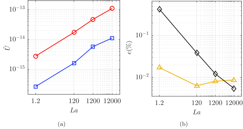
Fig. 16. Translating drop test case. Effect of the Laplace number La . (a) —○—, Maximum Velocity \tilde{U}_{max} ; —□—, RMS Velocity \tilde{U}_{RMS} . (b) —◇—, \Delta P_{max} ; —△—, \Delta P_{avg} , while keeping We = 0.4 and R/\Delta x = 12.8 .
