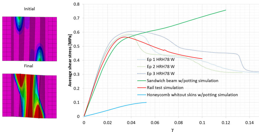
Fig. 27. Buckling of the cells and the average shear stress vs \gamma : three cases.
