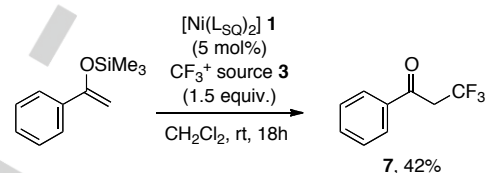
Scheme 1. Trifluoromethylation of a silyl enol ether by complex 1 . ^{19}\text{F} NMR yield was determined using fluorobenzene as internal standard.
