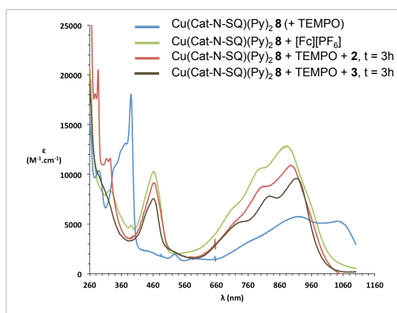
Figure 4. UV-vis spectra for TEMPO-trapping experiments of \text{CF}_3^+ source with complex 8 .
