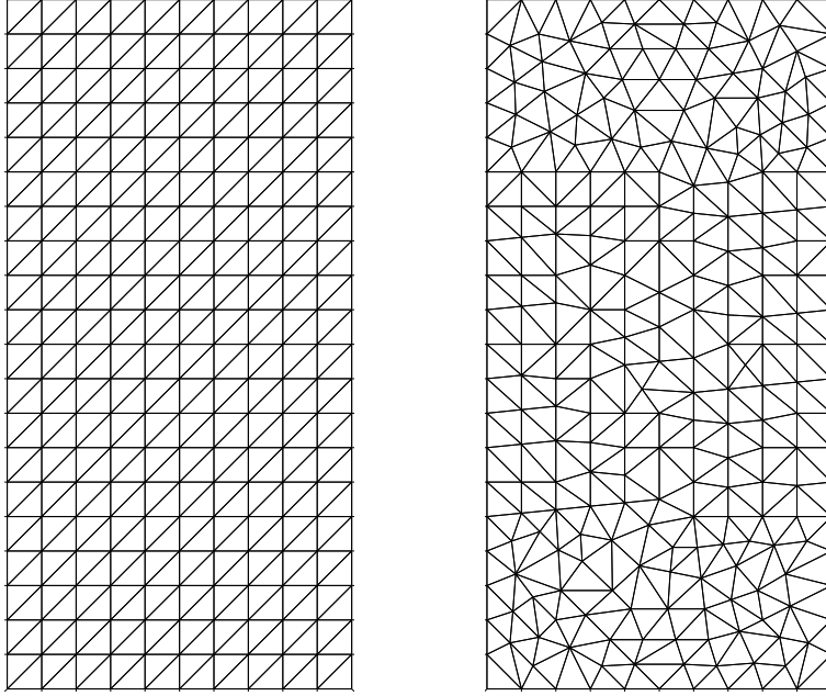
FIGURE 1. Regular meshes for Q_T ; Left: uniform mesh - h = 1.41 \times 10^{-1} . Right: non uniform mesh - h = 1.52 \times 10^{-1} .
