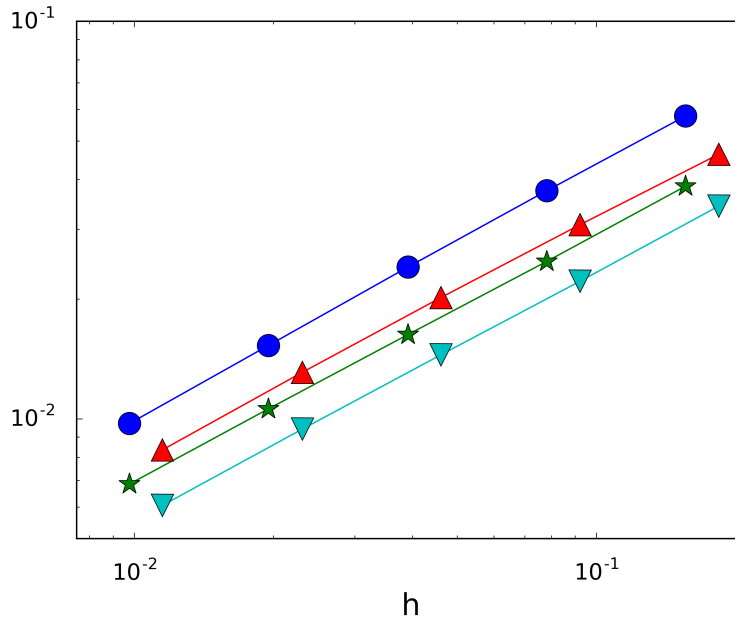
FIGURE 3. Evolution of \|v - \mathbf{q}_h(1, \cdot)\|_{L^2(0, T)} w.r.t h for uniform mesh with r = 1 ( \circ ), r = h ( \star ) and non uniform mesh with r = 1 ( \triangle ) and r = h ( \nabla ).
