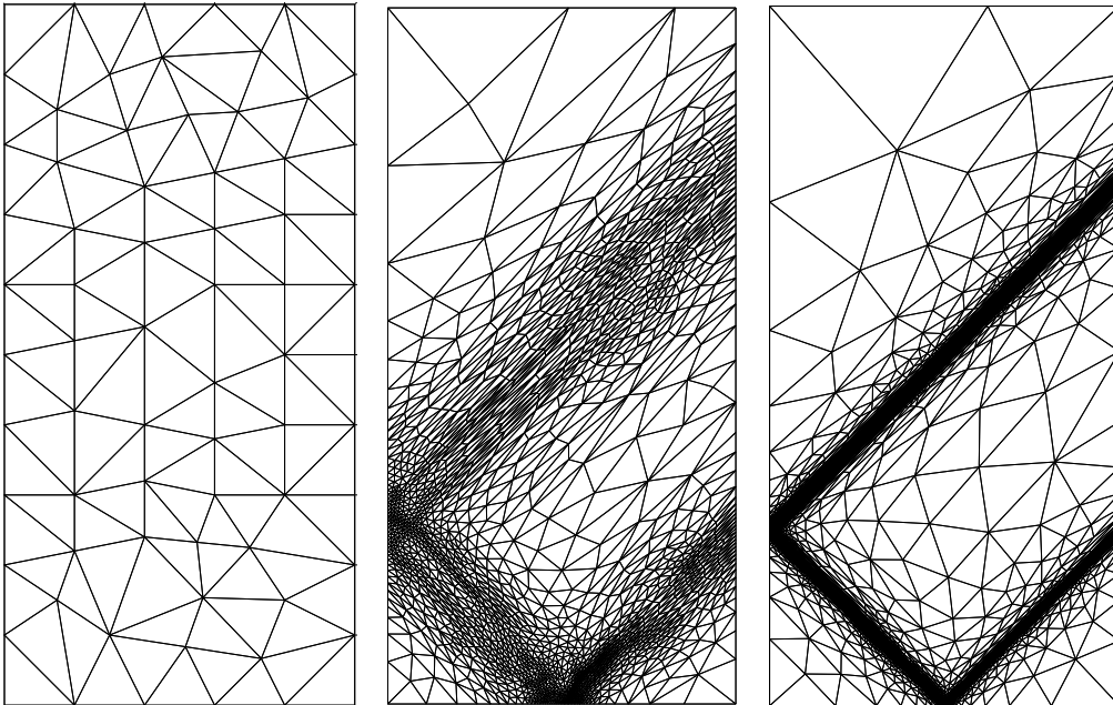
FIGURE 4. Iterative refinement of the triangular mesh over Q_T with respect to the variable \lambda_h : 110, 2880 and 8636 triangles.
