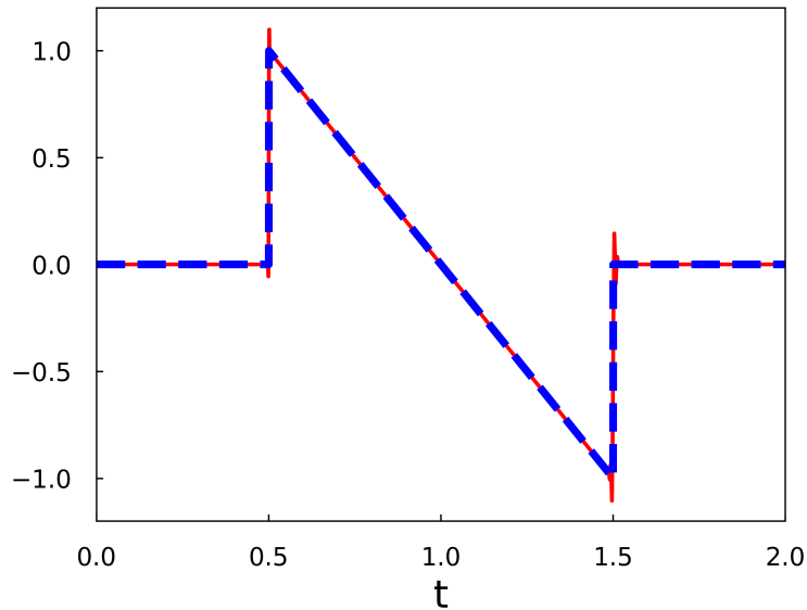
FIGURE 5. The primal variable \lambda_h in Q_T - Third adapted mesh in Figure 4, r = 10^{-6} .
