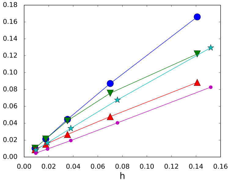
FIGURE 2. Non uniform mesh - Evolution of \sqrt{hr}\delta_h with respect to h (see Table 3) for r = 1 (○), r = 10^{-1} (▽), r = 10^{-2} (△), r = h (☆), r = h^2 (○).
