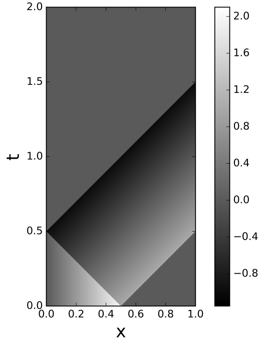
FIGURE 5. The primal variable \lambda_h in Q_T - Third adapted mesh in Figure 4, r = 10^{-6} .
